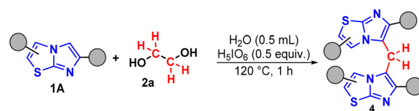
Scheme 3 Optimized protocol of methylenation of imidazo[2,1- b ]thiazole 1A . Conditions: 1A (0.3 mmol), 2a (0.5 molar equivalent), \text{H}_5\text{IO}_6 (0.5 equiv.), \text{H}_2\text{O} (0.5 mL), time (1 h), temperature ( 120^\circ\text{C} ).
