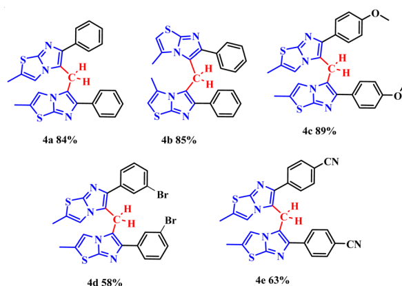
Fig. 3 Scope of imidazo[2,1- b ]thiazoles.
