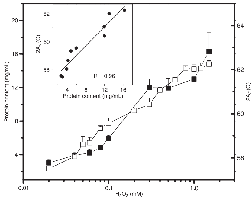
Figure 3. Protein content of the erythrocyte membranes (filled squares) and the electron paramagnetic resonance parameter, 2A_{//} , of 5-doxyl stearic acid in the erythrocyte membranes (open squares) as a function of H_2O_2 concentration. Insert. The linear correlation coefficient in the plot of protein content versus 2A_{//} was R = 0.96 .
