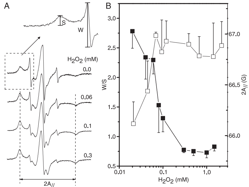
Figure 4. A, Electron paramagnetic resonance (EPR) spectra of 5-MSL bound to erythrocyte membrane proteins in the presence of gradually increasing H 2 O 2 concentrations. The relative intensities of the resonance lines S and W (the fraction of labels in the strongly and weakly immobilized components, respectively) are related to protein dynamics, as well as the 2A_{||} parameter (the separation between the vertical dotted lines in the magnetic-field unit). B, The W/S intensity ratio (filled squares) and the electron paramagnetic resonance parameter 2A_{||} (open squares) plotted as a function of H 2 O 2 concentration.
