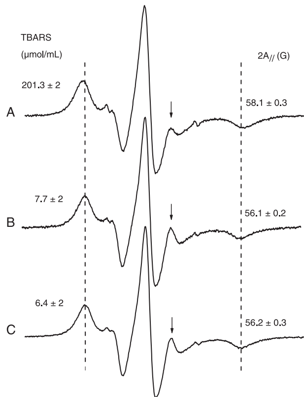
Figure 7. A, Electron magnetic resonance (EPR) spectrum of 5-doxy stearic acid in erythrocyte ghosts oxidized with 2 mM H_2O_2 and 200 \mu M FeSO_4 . B, Control sample (not oxidized). C, Samples pre-treated with 100 \mu M (+)-catechin and then oxidized as in A. The EPR parameter, 2A_{//} , increases for the oxidized sample, indicating a reduction in molecular dynamics or increased molecular order. The high-field resonance line of the inner hyperfine splitting (indicated by an arrow for each spectrum) decreases in the spectrum of oxidized membranes, indicating a loss of probe mobility. The figure also shows a decrease in the production of thiobarbituric acid reactive species (TBARS) resulting from lipid peroxidation of erythrocyte ghosts due to the antioxidant activity of (+)-catechin.
