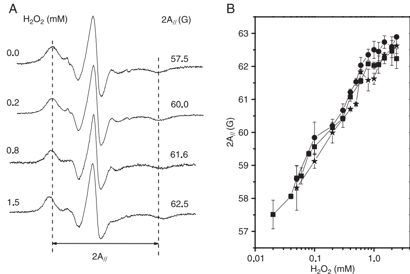
Figure 2. A, Electron paramagnetic resonance (EPR) spectra of 5-doxyl stearic acid in erythrocyte membranes in the presence of gradually increasing H_2O_2 concentrations. The vertical dotted lines are references for the control value of the 2A_{//} parameter, the outer hyperfine splitting. The total scanning range of the magnetic field of all spectra was 100 G. B, EPR parameter, 2A_{//} , for the control (squares), the 160- \mu M ascorbic acid-treated (circles) and the 300- \mu M \alpha -tocopherol-treated (stars) samples as a function of H_2O_2 concentration.
