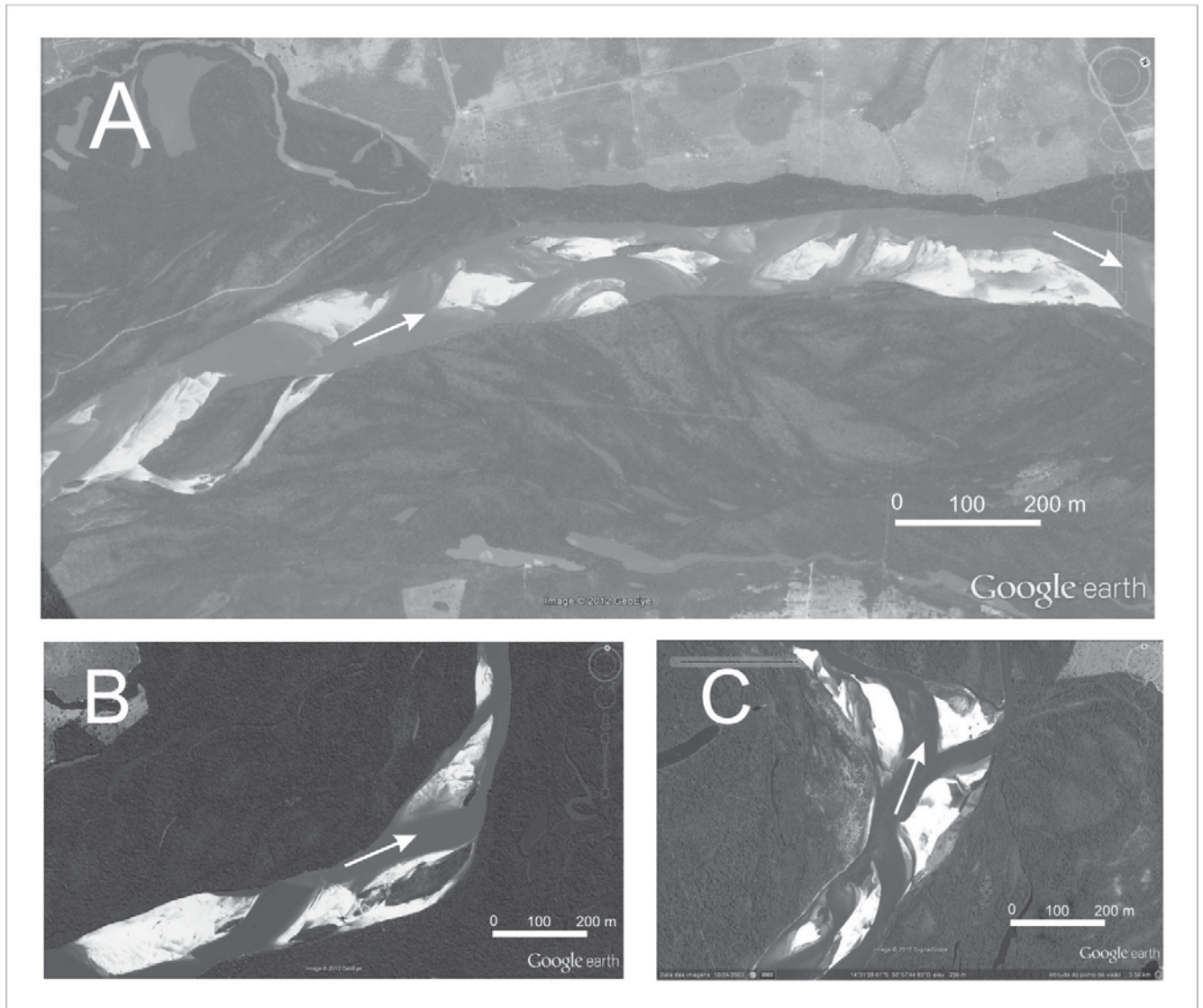
Figura 5 - Bancos de areias, centrais e laterais. Trechos com talvegue sinuoso a meandriforme: (A) S 14°49'42.24"/ W 51°05'15.36"; (B) S 14°58'46.56"/ W 51°09'08.64"; e, (C) S 14°31'7.68"/ W 50°57'28.84"
