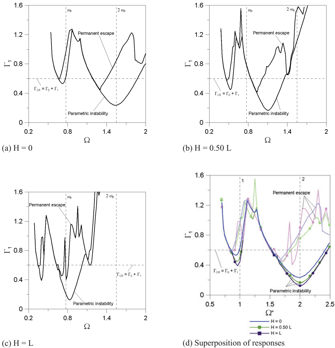
Figure 3: Parametric instability and escape boundaries for the axially pre-loaded cylindrical shell. ( \Gamma_0 = 0.40 ).
