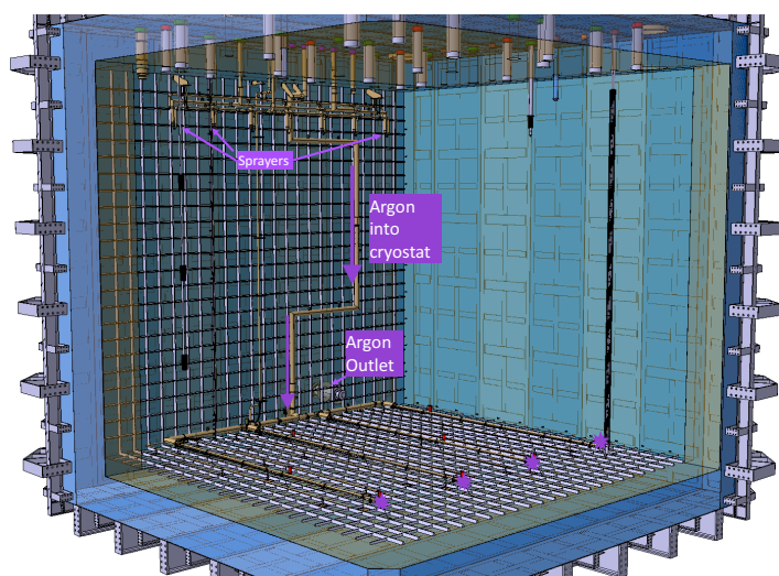
Figure 11. Cryogenics internal pipes and services.
