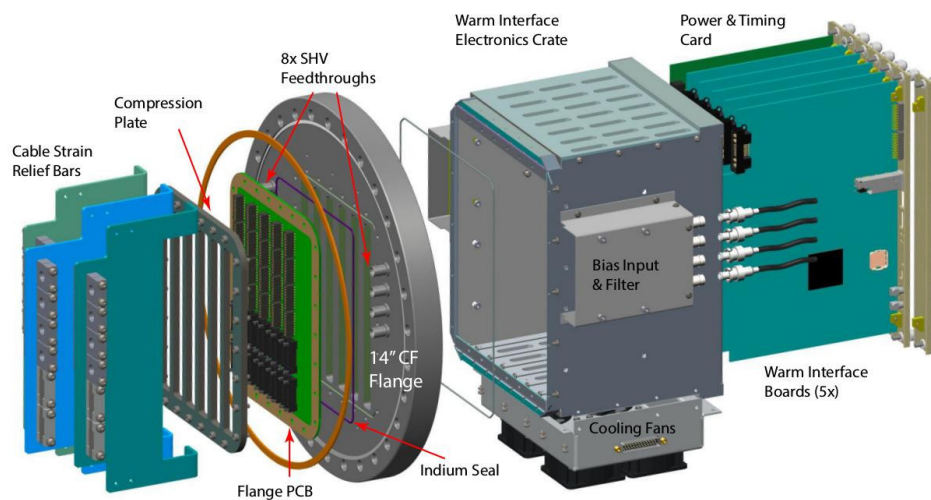
Figure 36. Exploded view of the ProtoDUNE-SP signal flange.
