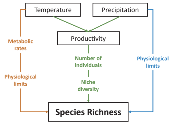
FIGURE 1 Path model depicting the analysed directional relationships and the underlying hypotheses linking different energy measures to species richness
