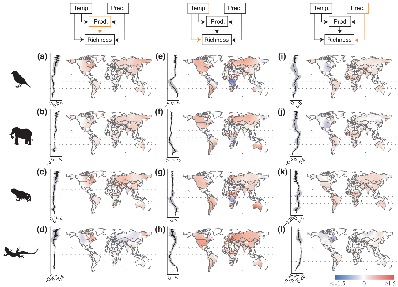
FIGURE 3 Direct coefficient strengths between species richness of terrestrial tetrapods and productivity (Prod.; a–d), temperature (Temp.; e–h) and precipitation (Prec.; i–l), according to the geographically weighted path model. Path coefficients are standardized and are mapped using the same colour scale, allowing direct comparison of their magnitudes. Silhouettes indicate the organism group for which the result is mapped. The full set of coefficient maps for all four taxonomic groups is available in the Supporting Information (Figures S4–S7). The line plot next to each map summarizes the path coefficient across latitude, plotted with the mean (black line) and the standard deviation (grey area). Dotted lines indicate the Tropic of Cancer, the Equator and the Tropic of Capricorn, respectively, from top to bottom. Silhouette images were taken from www.freepik.com
