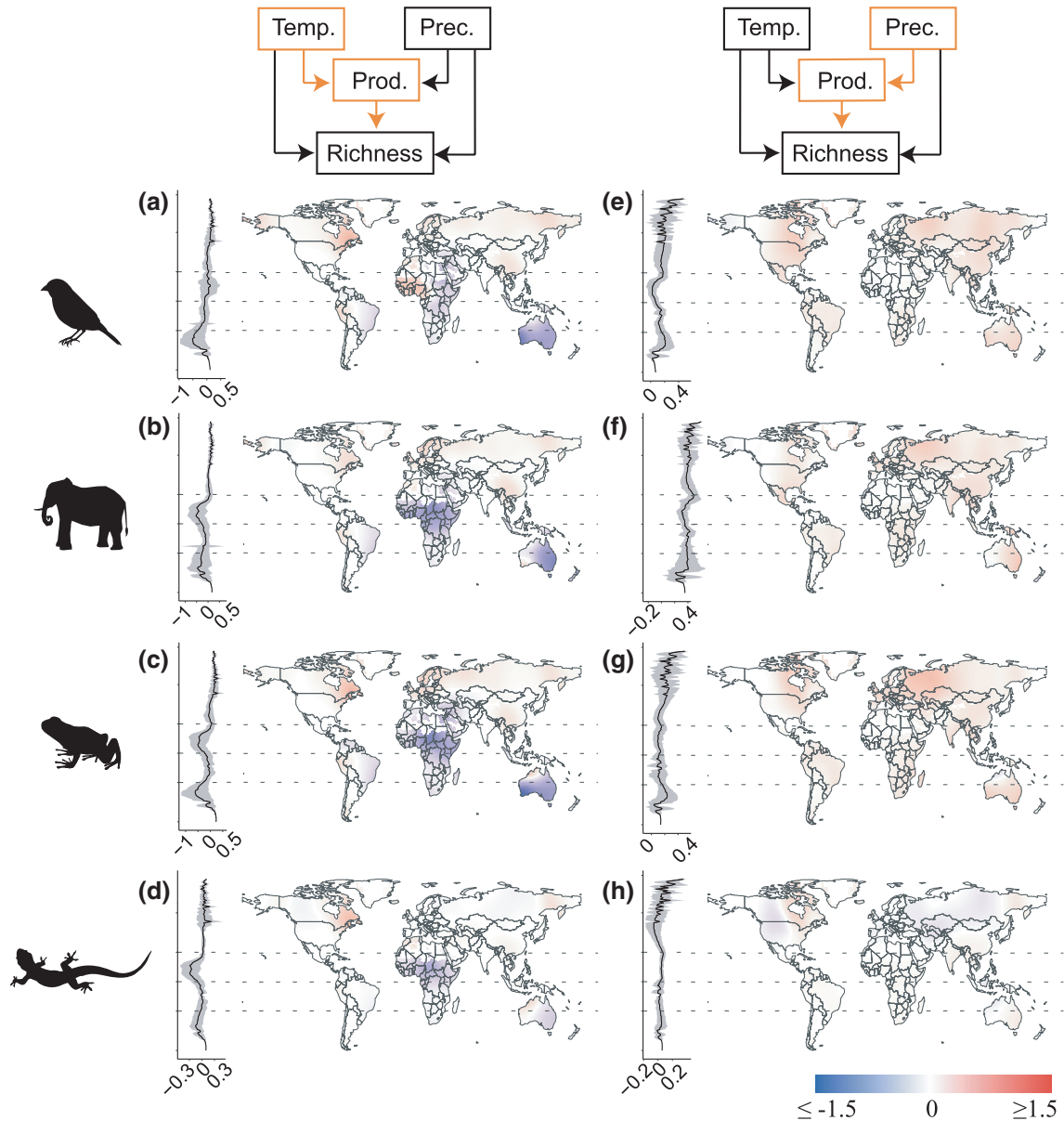
FIGURE 4 Indirect coefficient strengths between species richness of terrestrial tetrapods and temperature (Temp.; a–d) and precipitation (Prec.; e–h), according to the geographically weighted path model. Path coefficients are standardized and are mapped using the same colour scale, allowing direct comparison of their magnitudes. Silhouettes indicate the organism group for which the result is mapped. The full set of coefficient maps for all four taxonomic groups is available in the Supporting Information (Figures S4–S7). The line plot next to each map summarizes the path coefficient across latitude, plotted with the mean (black line) and the standard deviation (grey area). Dotted lines indicate the Tropic of Cancer, the Equator and the Tropic of Capricorn, respectively, from top to bottom. Silhouette images were taken from www.freepik.com
