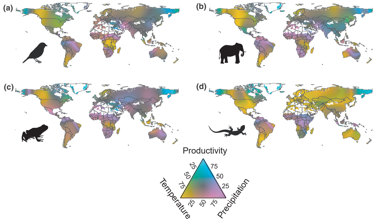
FIGURE 5 Relative importance of productivity, temperature and precipitation to the species richness of terrestrial tetrapods when considering both direct and indirect effects of temperature and precipitation through productivity. Colours indicate how much, as a percentage, a measure of energy is important to explain species richness based on the magnitude of the summed, standardized path coefficients. Shades of green indicate productivity, yellow temperature and pink precipitation as relatively more important. The black silhouette indicates the organismal group to which the result belongs. Silhouette images were taken from www.freepik.com
