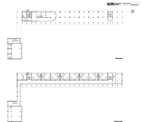
Fig. 26- Plantas do Narkomfin. Disponível em: https://socks-studio.com/2016/12/04/the-narkomfin-building-in-moscow-1928-29-a-built-experiment-on-everyday-life/ . Acesso em: 06 out. 2025
