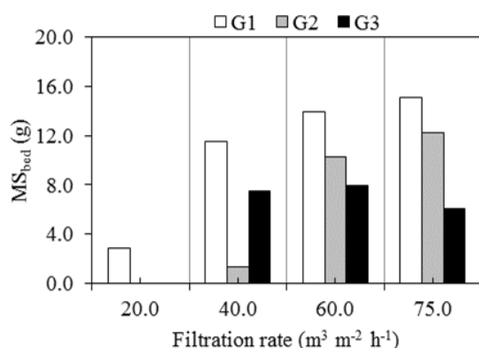
Fig. 11. Particle mass removed during the filtration process for all sand bed layers ( MS_{bed} ) (g) for sand particle sizes (G1, G2 and G3) combined with different filtration rates (FR20, FR40, FR60 and FR75) considering the average among filtration cycles (C1, C2 and C3).
