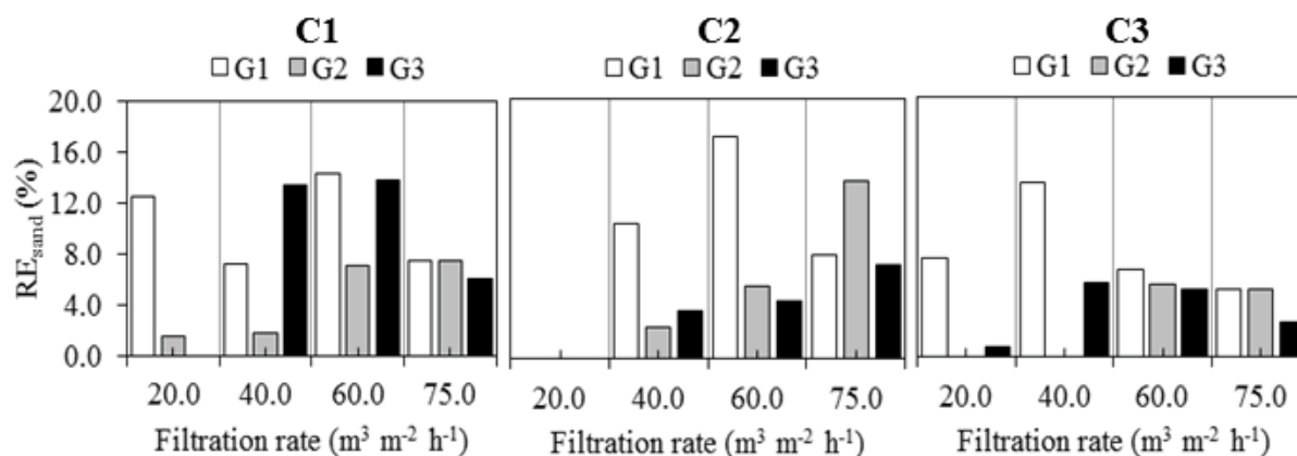
Fig. 12. Performance of filtration removal efficiency using TSS values of the sand ( RE_{sand} ) (%) for different combinations of filtration rates, sand particle sizes and filtration cycles.
