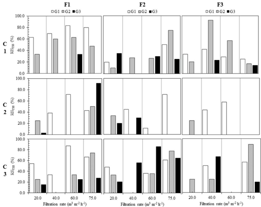
Fig. 4. Filtration removal efficiency using TSS from water samples ( RE_{TSS} ) (%) considering the first sampling (0 min) calculated for different sand particle size and filtration rate combinations for the filtration cycles C1, C2 and C3.
