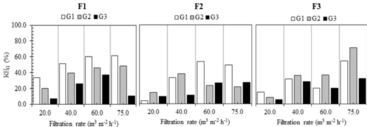
Fig. 7. Filtration removal efficiency using TSS from water samples considering all data collected for time and filtration cycles ( RE_G ) (%) for different sand particle sizes and filtration rates ( m^3 m^{-2} h^{-1} ).
