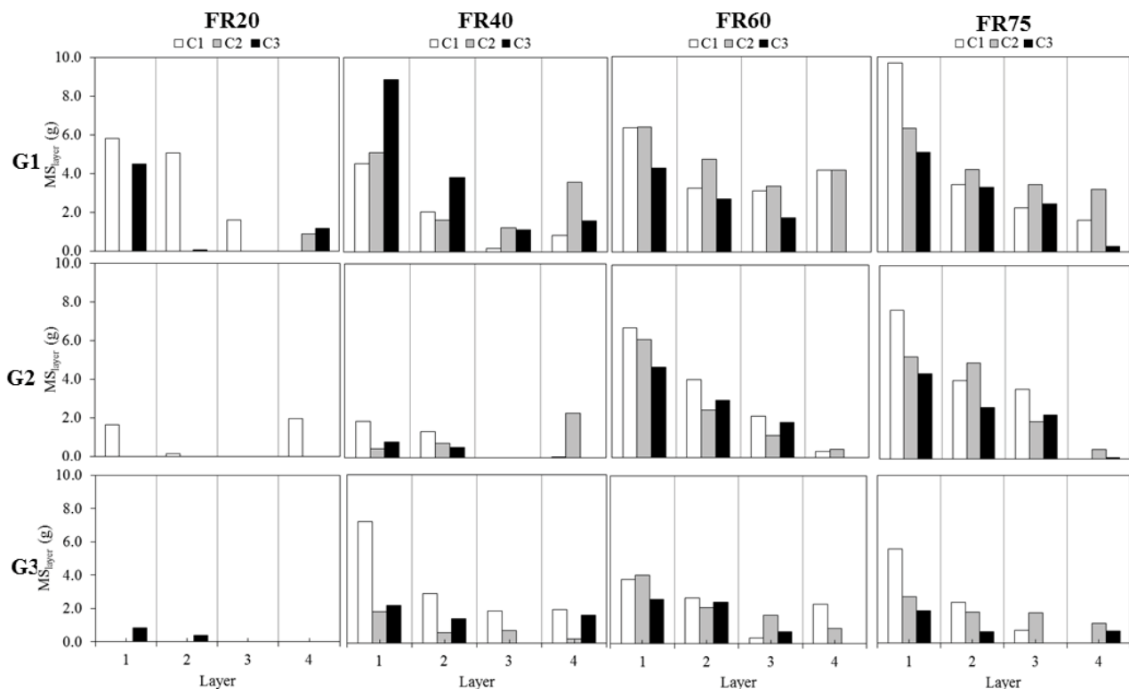
Fig. 9. Particle mass removed during the filtration process from different sand bed layers ( MS_{layer} ) (g) for sand particle sizes (G1, G2 and G3) combined with different filtration rates (FR20, FR40, FR60 and FR75) and cycles (C1, C2 and C3).
