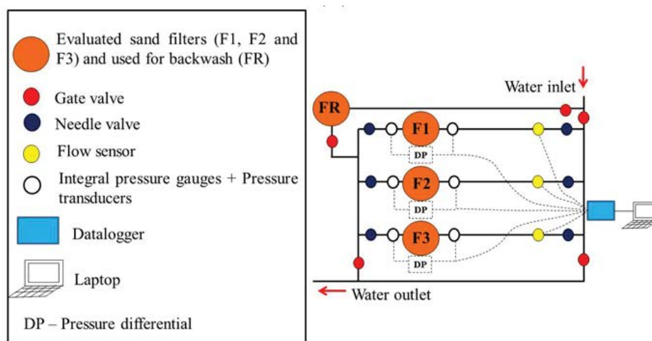
Fig. 1. Experimental setup and monitoring devices.
