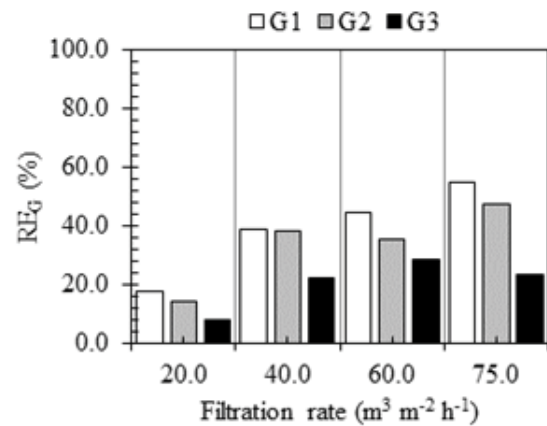
Fig. 8. Filtration removal efficiency calculated considering TSS from water samples and data collected for times and filtration cycles ( RE_G ) (%) for different sand particle sizes and filtration rates ( m^3 m^{-2} h^{-1} ) according to the average value between sand filters.
