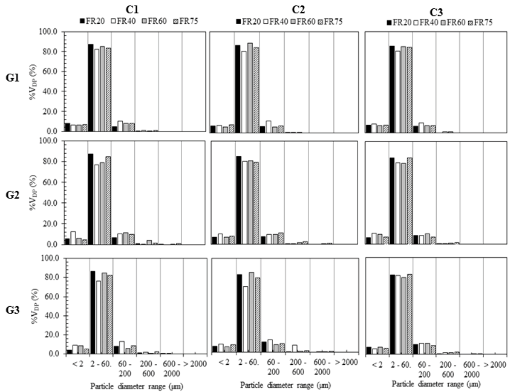
Fig. 3. Volume average percentage of different particle diameters contained in inlet water.
