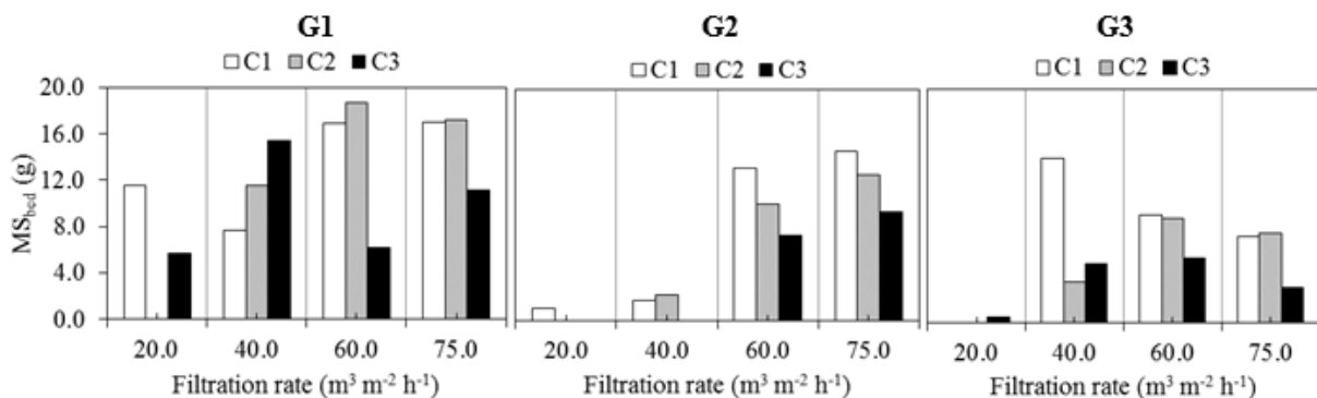
Fig. 10. Particle mass removed during the filtration process for all sand bed layers ( MS_{bed} ) (g) for all sand particle sizes (G1, G2 and G3) combined with different filtration rates (FR20, FR40, FR60 and FR75) and cycles (C1, C2 and C3).
