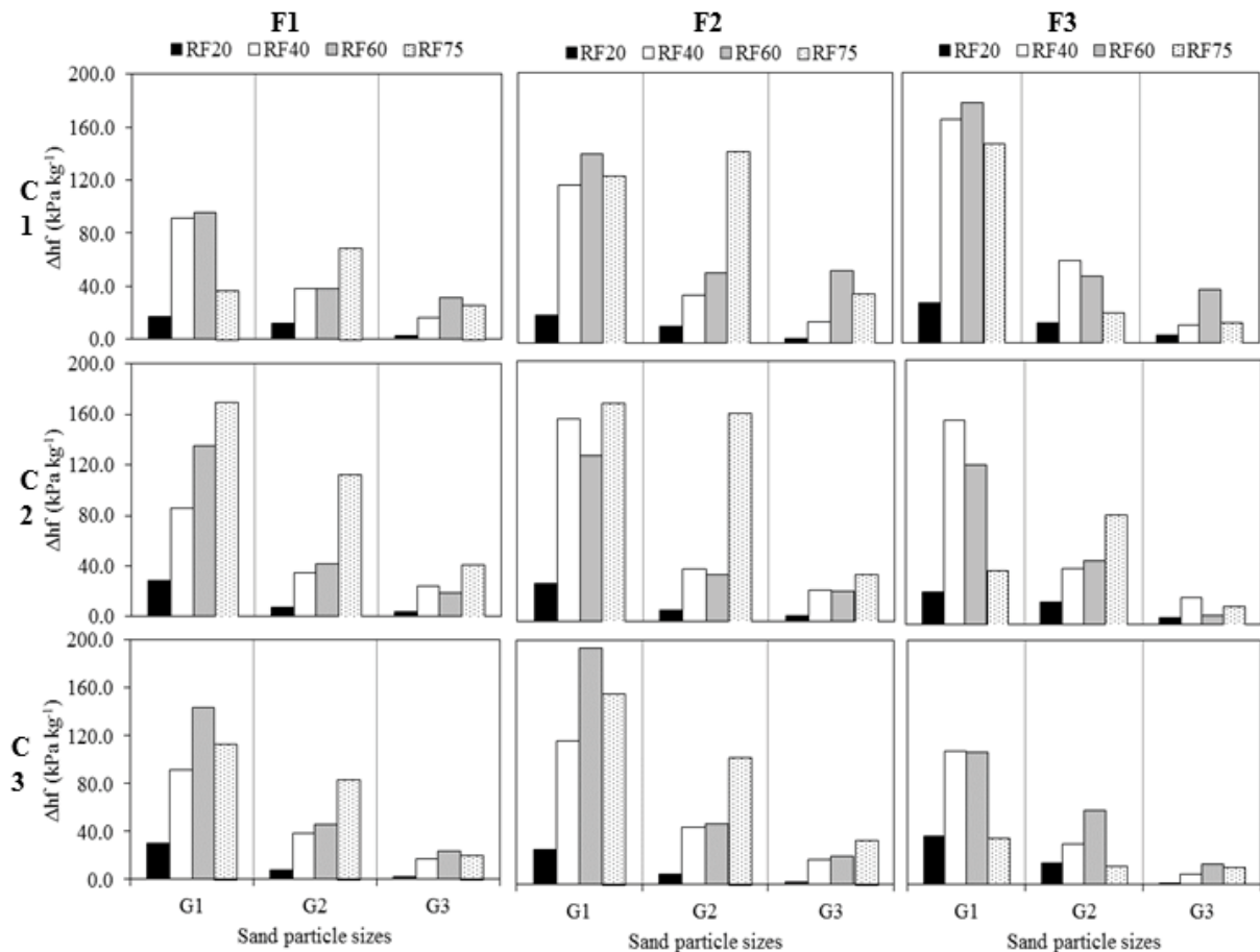
Fig. 13. Behavior of increase in filter head loss of the sand filter weighted by total suspended solids caught at each evaluation.
