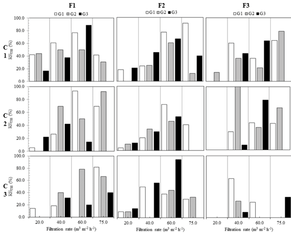
Fig. 5. Filtration removal efficiency using TSS from water samples ( RE_{TSS} ) (%) considering the second sampling (120 min) for different sand particle size and filtration rate combinations for the filtration cycles C1, C2 and C3.
