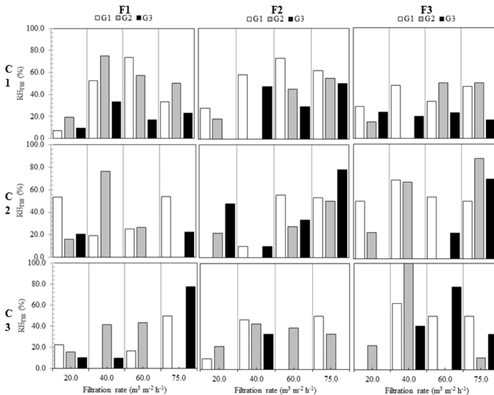
Fig. 6. Filtration removal efficiency using TSS from water samples ( RE_{TSS} ) (%) considering the third sampling (240 min) for different sand particle size and filtration rate combinations for the filtration cycles C1, C2 and C3.
