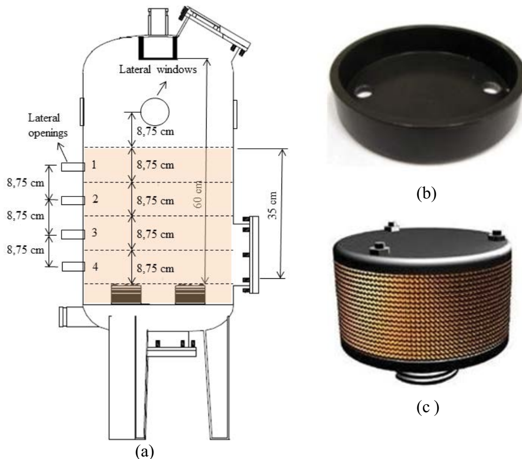
Fig. 2. Evaluated sand filter. Detail of the structural modification (side openings and windows) and their locations (a); diffuser plate with lid (b) and underdrains (c).
