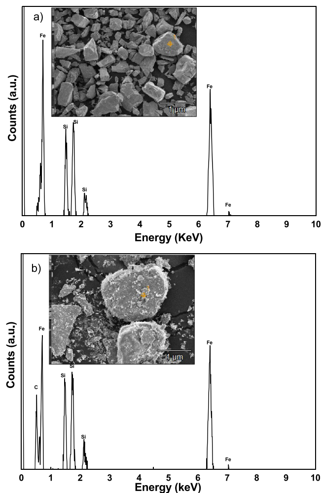
Figure 2. SEM–EDX analysis for (a) FeSi and (b) FeSi@5%SiC powders.
