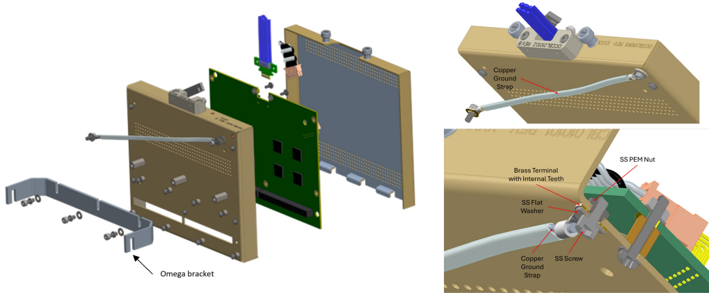
Figure 8. Drawing of how a FEMB is assembled into its enclosing CE box, including a ground strap and omega bracket used for mounting onto an APA. Details of the ground strap connection to the CE box are shown on the right.
