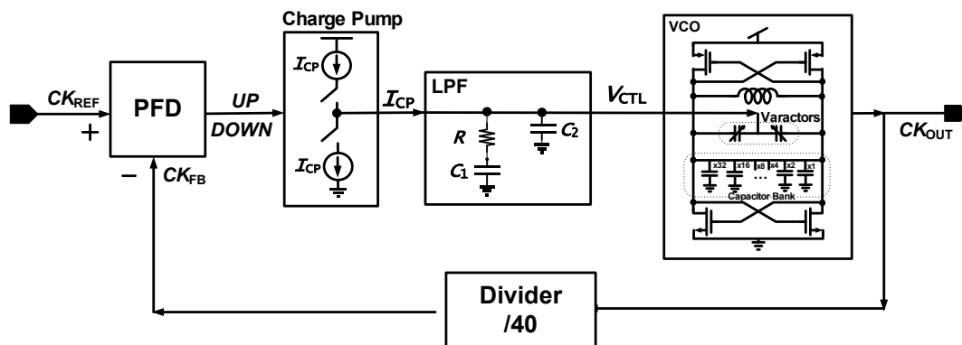
Figure 5. Block diagram of the COLDATA PLL, which generates a 2.5 GHz clock for use by the data serializers. The phase and frequency detector (PFD) takes the 62.5 MHz reference clock and the PLL’s feedback clock as input. The differences are used to produce UP and DOWN signals used as input to the charge pump, which uses a tunable bias current I_{CP} . The charge pump output goes through a low-pass filter (LPF), which uses a tunable bias current I_{CP} . The charge pump output goes through a low-pass filter (LPF) before being used to drive the voltage-controlled oscillator (VCO), which produces the output clock. The feedback clock is extracted from this output with a divide-by-40 circuit, which cuts the 2.5 GHz output back down to match the 62.5 MHz input clock.
