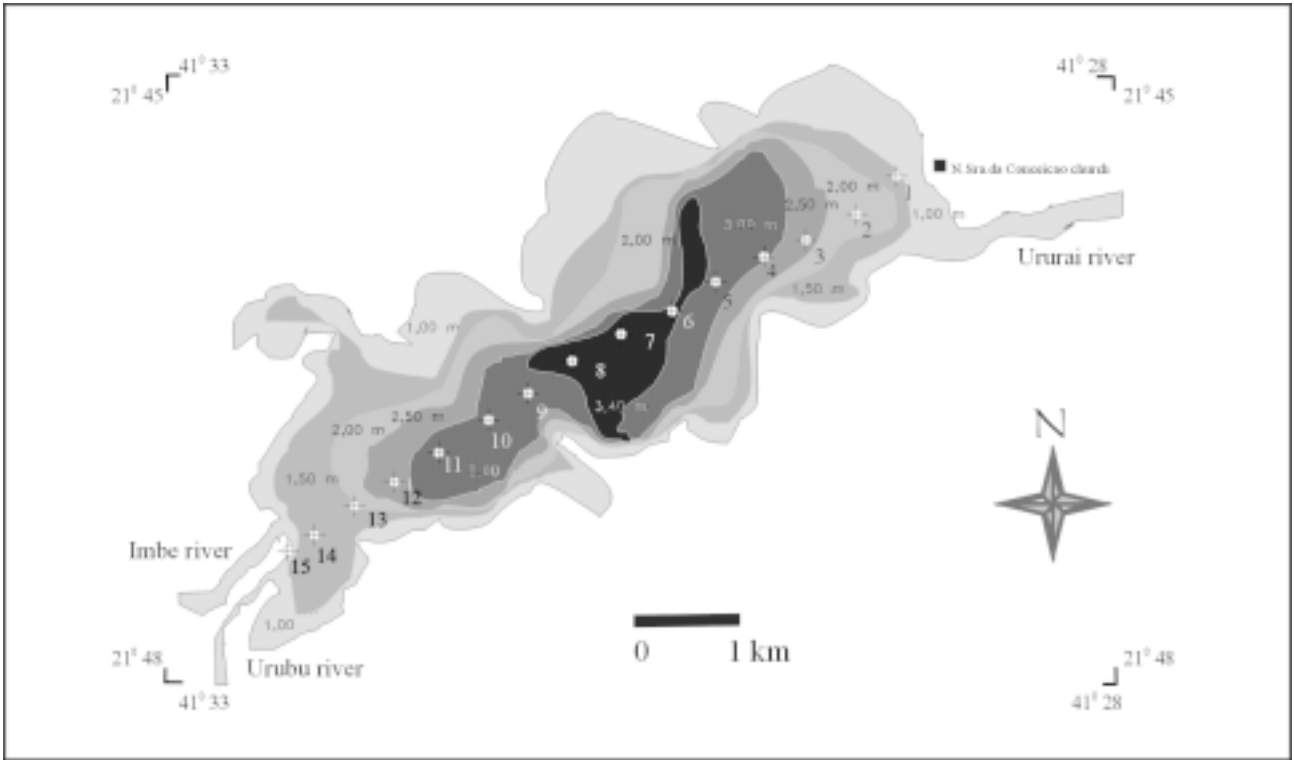
Figure 2 - Topography map of the bottom of the Lagoa de Cima lake and localization of each point sampled (modified from PROAGRO, 1975).
