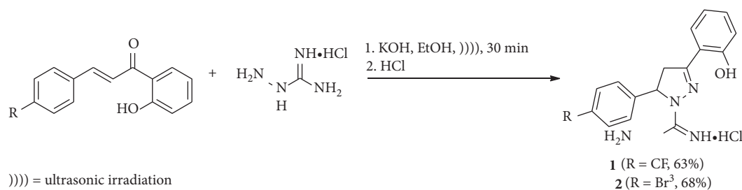
SCHEME 1: Ultrasound-promoted synthesis of pyrazoline hydrochlorides.
