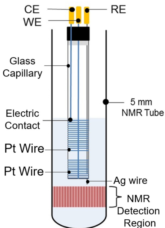
Fig. 1. Electrochemical cell and electrodes. The working, counter and reference electrodes were fixated on a glass capillary tube. The miniaturized electrodes were inserted into a standard 5 mm NMR tube and positioned 0.5 mm above the detection region.
