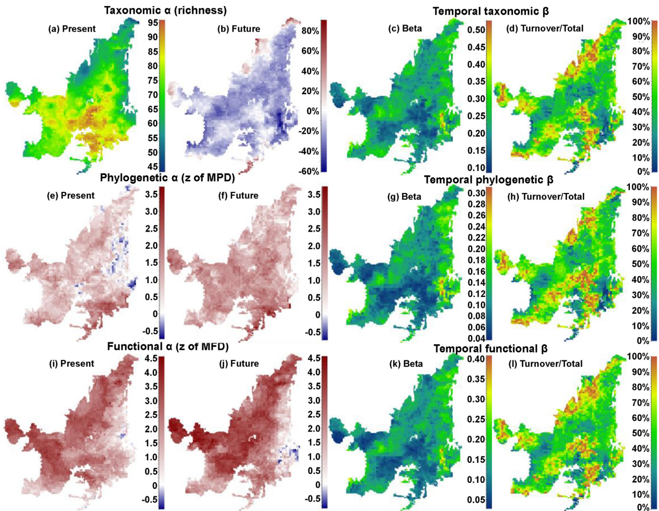
Fig. 1. On the left side, maps indicating the present values and the percentages of increase or decrease (future–present) in values of taxonomic alpha diversity (“a” and “b” for richness), and present and future values phylogenetic (“e” and “f” for z of MPD), and functional (“i” and “j” for z of MFD) structures. On the right side, maps indicating the temporal beta diversity and percentage of turnover (out of total beta diversity) of taxonomic (“c” and “d”), phylogenetic (“g” and “h”), and functional (“k” and “l”) beta diversities between present time and the near future. Future values were calculated for the year of 2070 under a scenario of intermediate concentration of greenhouse gases (RCP 6.0).
