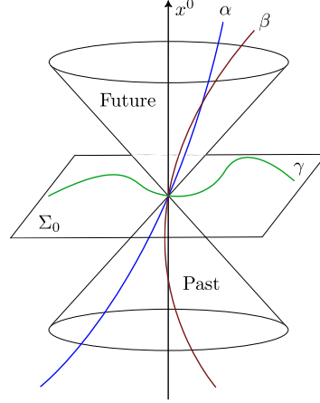
Figure 3.2: A light-cone oriented by the x^0 axis. The red and blue lines are timelike world lines, since they are in the light-cone causal region. But the green one is out of this region, so we call it spacelike world line. Also, note that, the region \Sigma_0 is a spatial hypersurface where all points on it are simultaneous, relative to x^0 , and no timelike world line can pass through it more than one time. Thus, \Sigma_0 is a Cauchy Surface.
