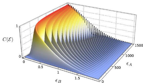
Figure 5.5: Dependence of the Channel Capacity with the coupling constants \epsilon_A and \epsilon_B . (Source: I. B. Barcellos and A. G. Landulfo, “Relativistic quantum communication: energy cost and channel capacities”)
