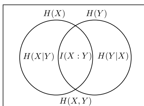
Figure 2.1: Given the random variables X and Y , the relations between the associated information measures are described by the joint entropy, conditional entropy and also the mutual information. From this illustration we can see how these measurements are related to each other. (Source: V. Vedral et al., Introduction to quantum information science , 2006)
