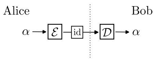
Figure 2.2: Alice encodes the message " \alpha ", using the encoder \mathcal{E} , to a codeword "00" which is transmitted by the noiseless bit channel (indicated by "id") to Bob. The last step decodes the same message sent by Alice.
