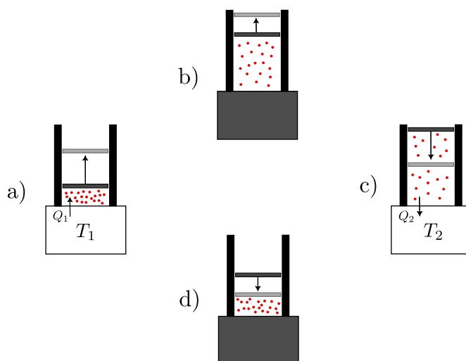
Figure 5.2: The Carnot Cycle. Where, a) describes a reversible isothermal expansion of the gas, b) is the reversible adiabatic expansion, c) represents the reversible isothermal compression and d) illustrates the reversible adiabatic compression. Note that there is only one piston on the system, which is the dark grey bar, the lighter one represents the final position of the piston.
