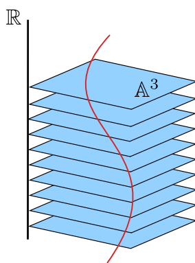
Figure 3.1: Newtonian causal structure of spacetime.
