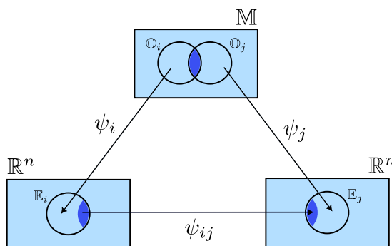
Figure 3.3: Representation of the maps \psi_i , \psi_j and \psi_{i,j} .
