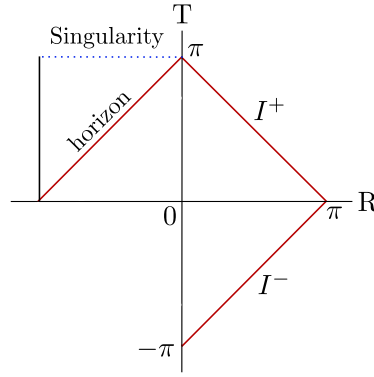
Figure 4.3: Penrose diagram with a singularity.
