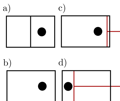
Figure 5.1: The process of erasing the information about a molecule's initial position. Fig. b) is the box without the partition, c) represents the box with a piston and d) is the process of moving it, changing the molecule's position.
