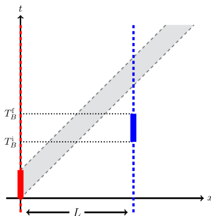
Figure 5.6: Causal relation between the emission and detection events. (Source: I. B. Barcellos and A. G. Landulfo, “Relativistic quantum communication: energy cost and channel capacities”)
