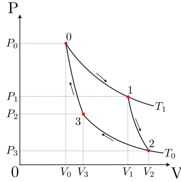
Figure 5.4: (P, V) diagram of the Carnot cycle.
