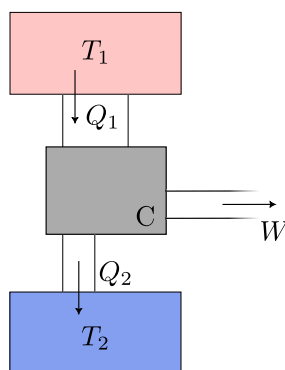
Figure 5.3: Representation of a Carnot engine C operating with two reservoirs.
