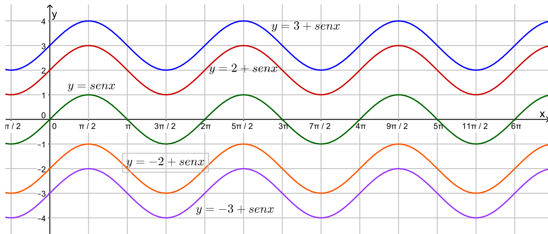
Figura 3: f(x) = \text{sen } x Comparada com f(x) = a + \text{sen } x
