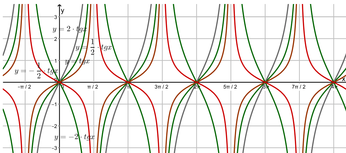
Figura 18: f(x) = \operatorname{tg} x Comparada com f(x) = b \operatorname{tg} x
