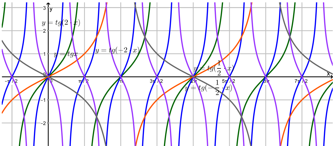
Figura 19: f(x) = \text{tg} x Comparada com f(x) = \text{tg}(cx)
