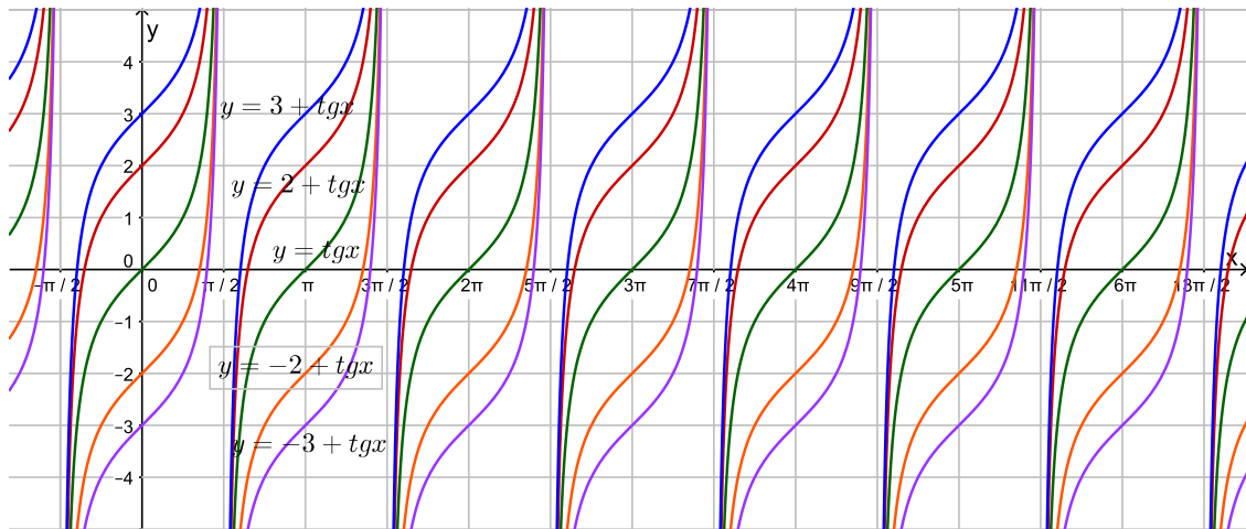
Figura 17: f(x) = \operatorname{tg} x Comparada com f(x) = a + \operatorname{tg} x
