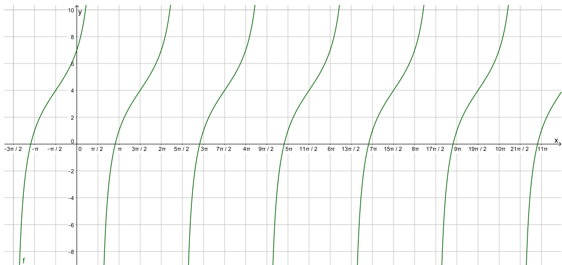
Figura 22: Gráfico de f(x) = 4 + 3 \operatorname{tg}\left(\frac{1}{2}x + \frac{\pi}{4}\right)
