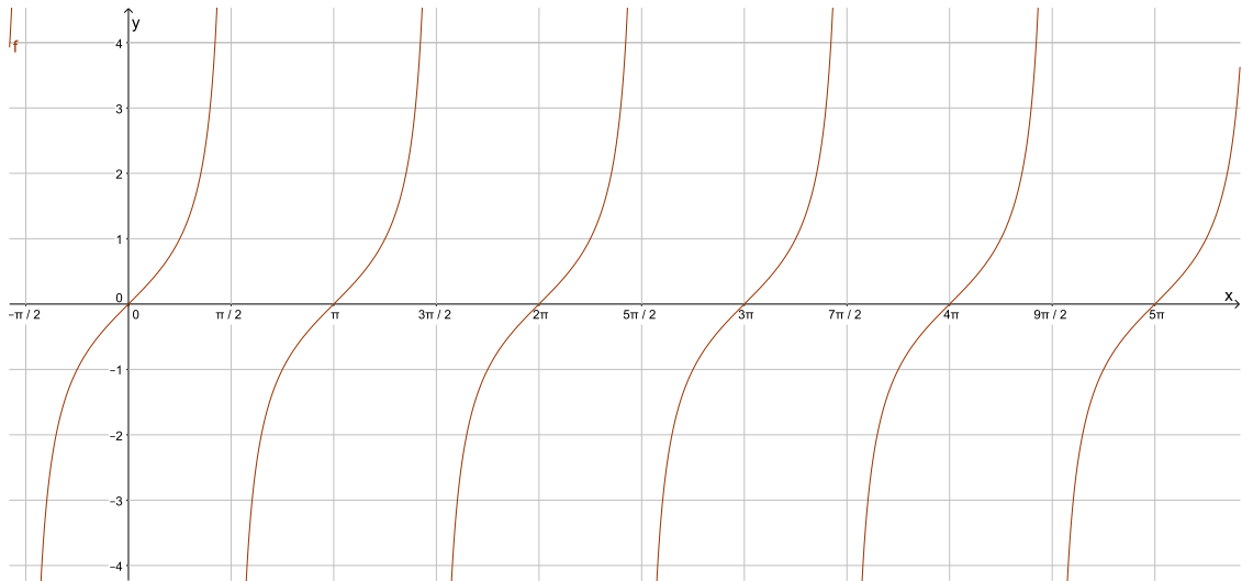
Figura 16: f(x) = \text{tg } x
