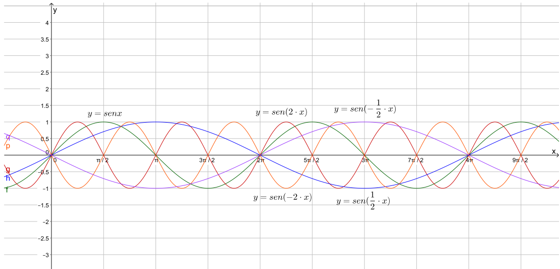
Figura 5: f(x) = \text{sen } x Comparada com f(x) = \text{sen}(cx)
