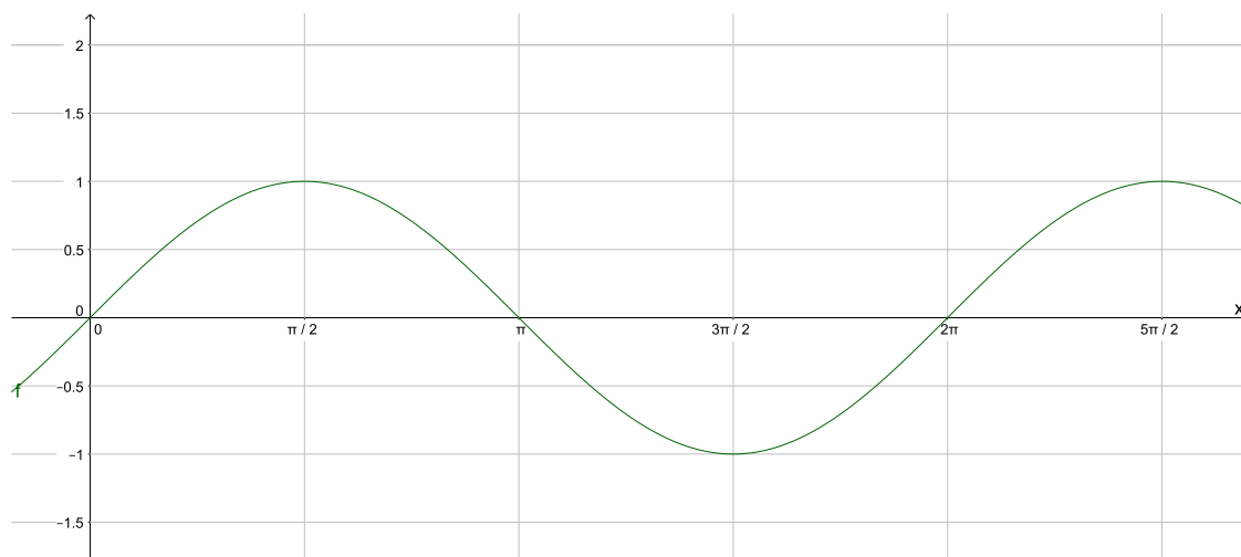
Figura 2: f(x) = \text{sen } x
