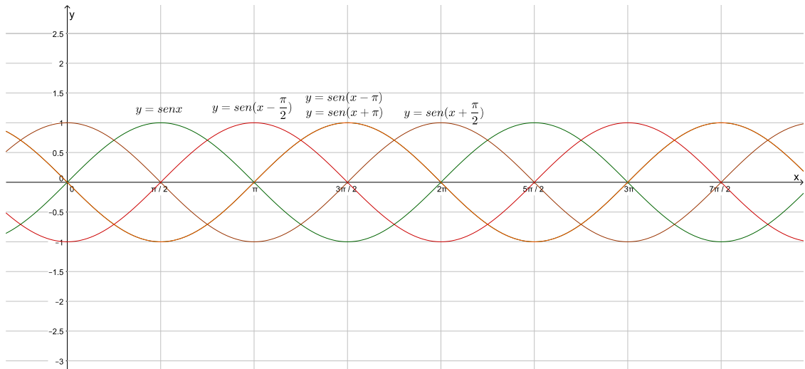
Figura 7: f(x) = \text{sen } x Comparada com f(x) = \text{sen}(x + d)
