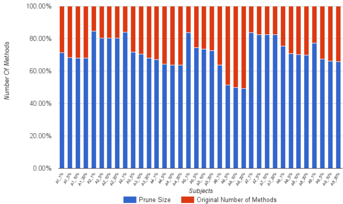
Figure 5.1: Prune size in the subjects for each time constraint.
