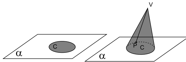
Figura 15: Cone Circular
