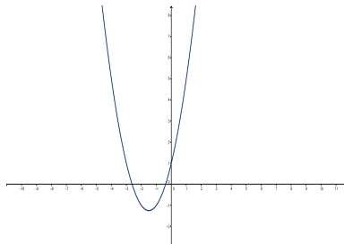
(a) b > 0
